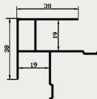
18' LİK ÇAVUŞ (ALÜMİNYUM) 18- CHEVRON PROFILE (ALUMINUM)
