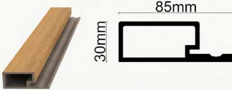
VEGA BİTİŞ PROFİLİ (WPC) VEGA FINISH PROFILE (WPC)
