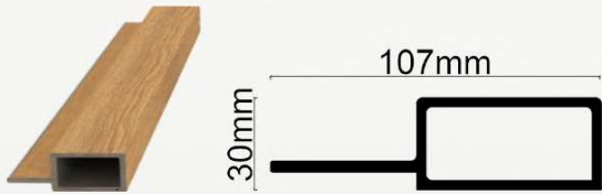
VEGA BİTİŞ PROFİLİ (WPC) VEGA FINISH PROFILE (WPC)
