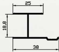
18' LİK ÇAVUŞ (ALÜMİNYUM) 18- CHEVRON PROFILE (ALUMINUM)
