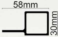
TRİO BİTİŞ PROFİLİ (PVC) TRİO FINISH PROFILE (PVC)
