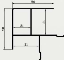
30' LUK ÇAVUŞ (ALÜMİNYUM) 30- CHEVRON PROFILE (ALUMINUM)
