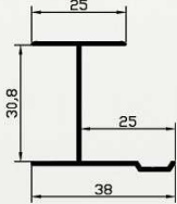
30' LUK ÇAVUŞ (ALÜMİNYUM) 30- CHEVRON PROFILE (ALUMINUM)
